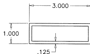
16 REINF. TUBE
