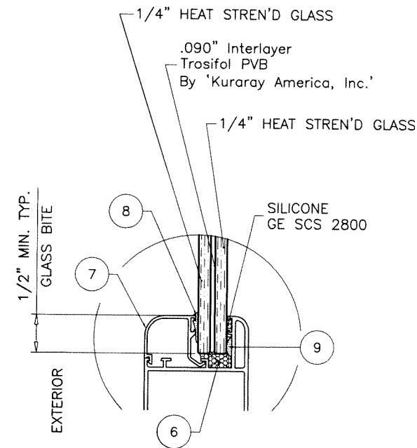
GLAZED DOOR 9/16" OVERALL LAM. GLASS
