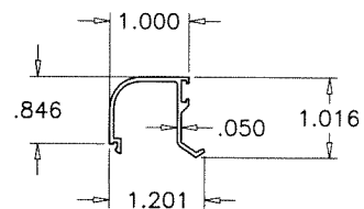
7 GLAZING BEAD
