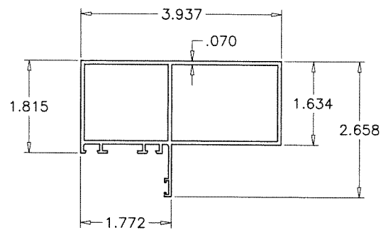
1 FRAME HEAD/JAMB
