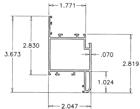
2 LEAF RAIL/STILE
